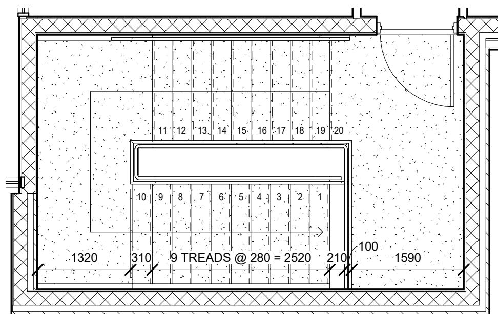
2 SECOND FLOOR PLAN 1:50 A-4
