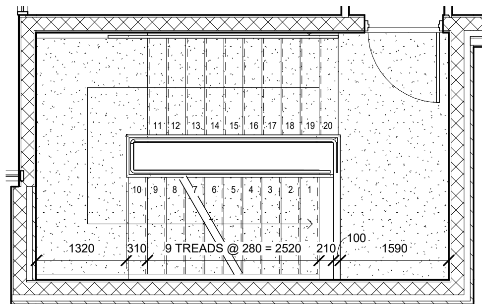
4 SECOND FLOOR PLAN 1:50 A-4
