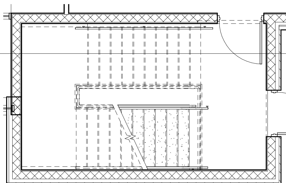
3 FIRST FLOOR PLAN 1:50 A-4
